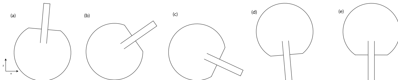
Figure 2. Phases I to V of the Tippe top's motion, shown in the xz -plane
