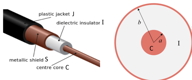
Diagram of a coaxial cable showing C - the centre core, I - the dielectric insulator, S - the metallic shield and J - the plastic jacket.
