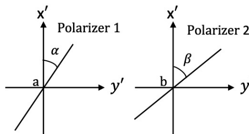
Fig. 3: Two linear polarizers 1 and 2 for coincidence measurement of photons that pass a and b .
