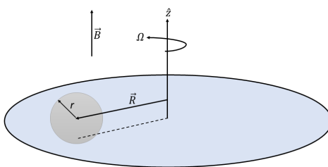
Figure 2. Ball rolling on the turntable in a constant magnetic field \vec{B}
